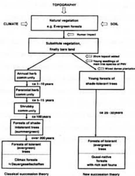
Fig. 4. Comparison between the classical succession theory and the new succession theory in forest bare area of Japan.
